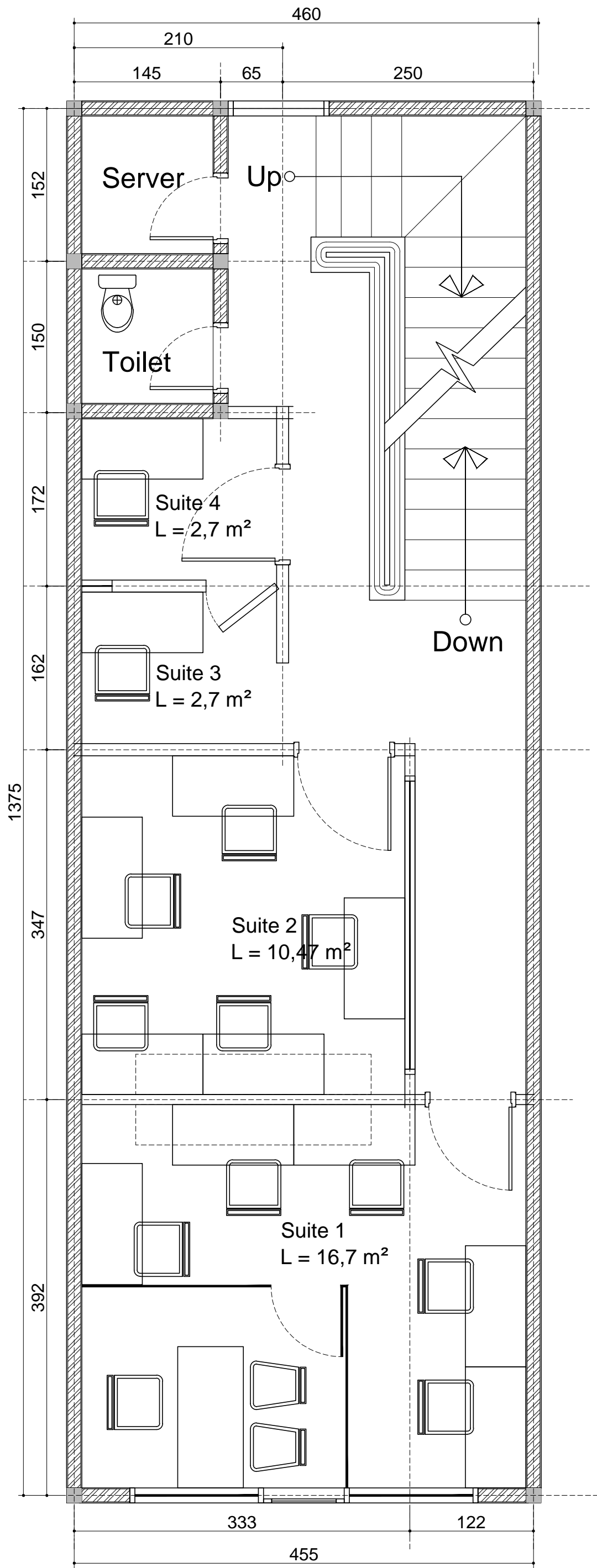
02 | Second Floor Plan A 01 | 01 | Skala 1 : 50
