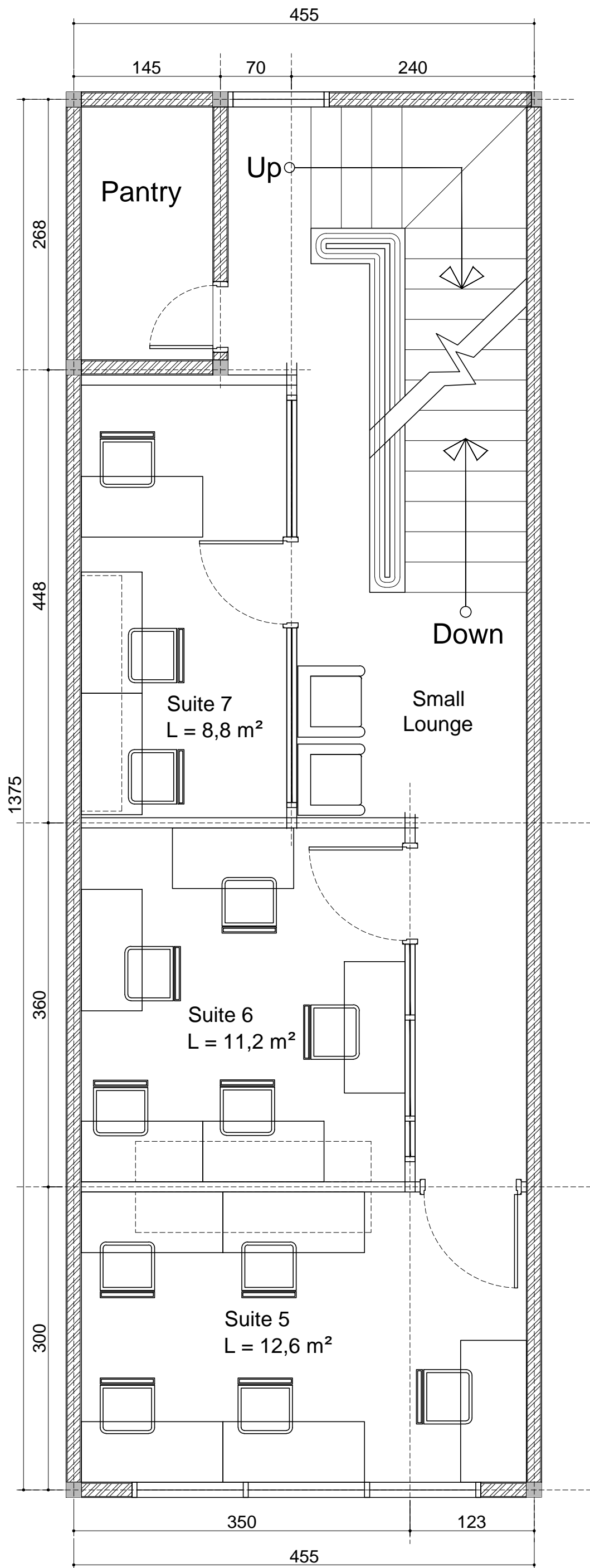
03 Third Floor Plan A 01 | 01 Skala 1 : 50
