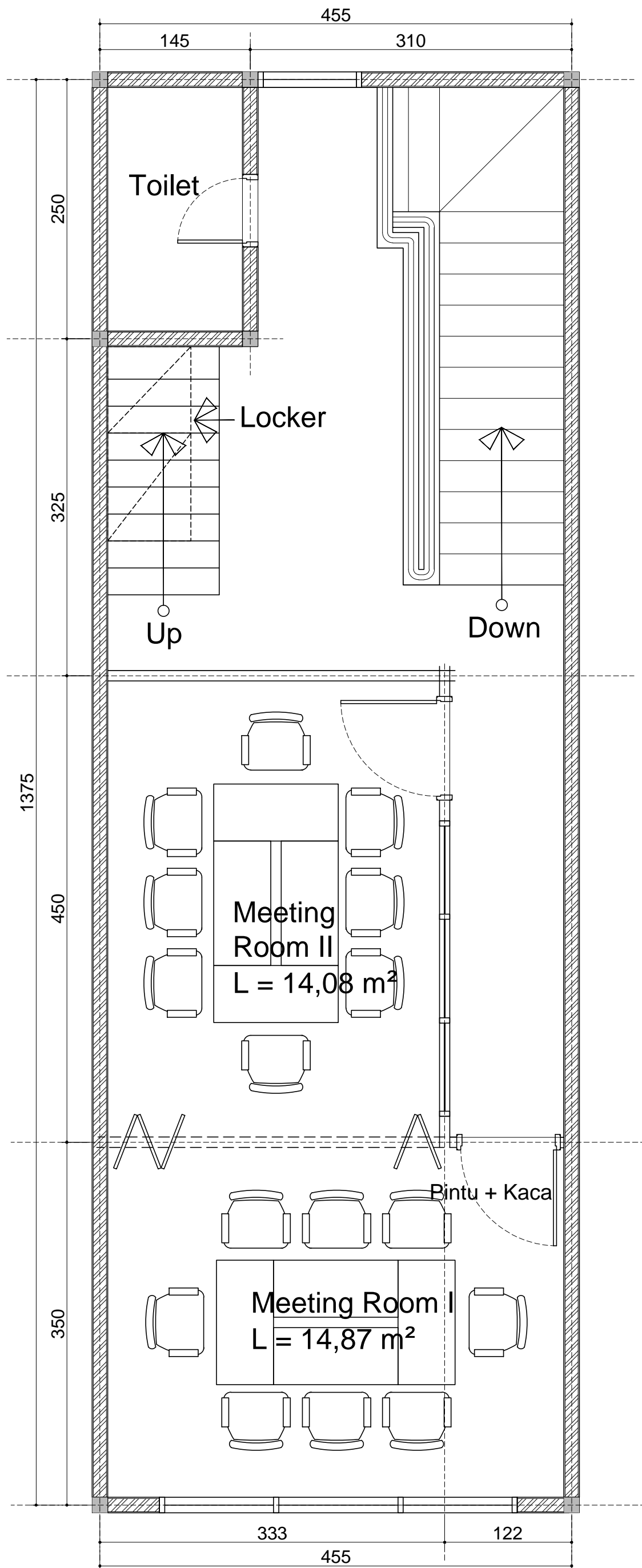
04 Fourth Floor PPlan A 01 | 01 Skala 1 : 50
